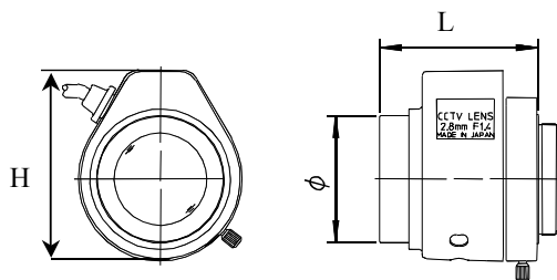
Auto iris: Video drive - Direct drive
