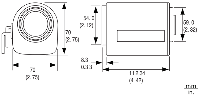
Dimensions LTC 3384/21
